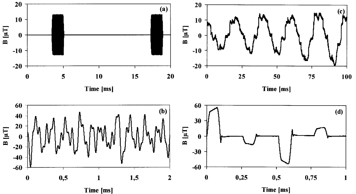
Fig. 2. Representative examples for broadband and pulsed magnetic fields. a) Burst of sinusoidal magnetic field oscillations measured inside an anti-theft gate; b) Simulated magnetic field consisting of seven non-coherent sinusoidal components; c) AC magnetic field measured in the vicinity of an industrial switched power source for high power electric motors; d) Magnetic field pulses measured inside a metal detector gate. Waveforms (a) and (c) were obtained from Jokela (2000).
