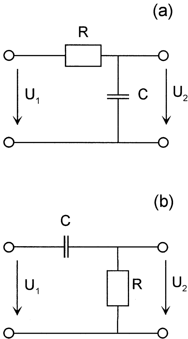
Fig. 4. Simple RC circuits for the weighting of dB/dt (a) and B (b).
