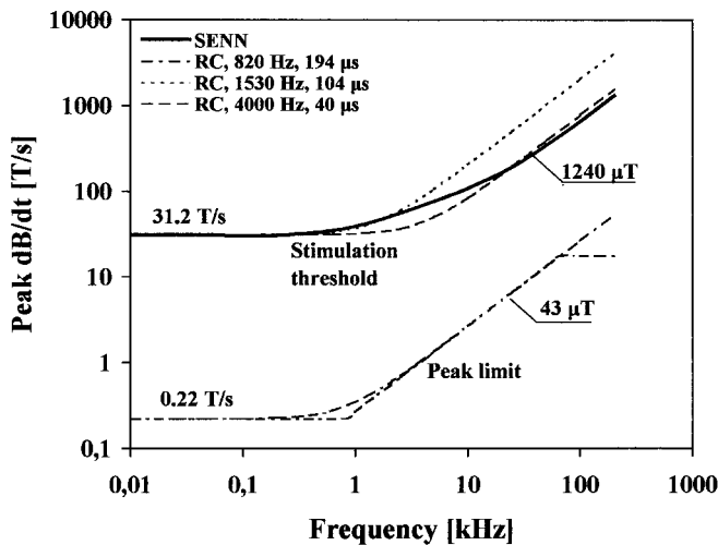
Fig. 3. Stimulation threshold and peak limit for a sinusoidal magnetic field as a function of frequency (Jokela 2000). The solid curve shows the stimulation threshold calculated with the SENN (spatially extended nonlinear nodal) model of Reilly (1998). The lower curve is the peak limit for occupational exposures.
