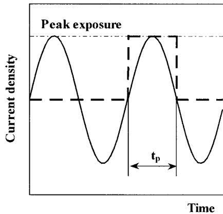
Fig. 1. Equivalent sinusoidal waveform for the determination of the peak restriction for a rectangular current density pulse.
